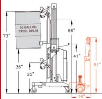
#240156 / #240157 SCHEMATIC
