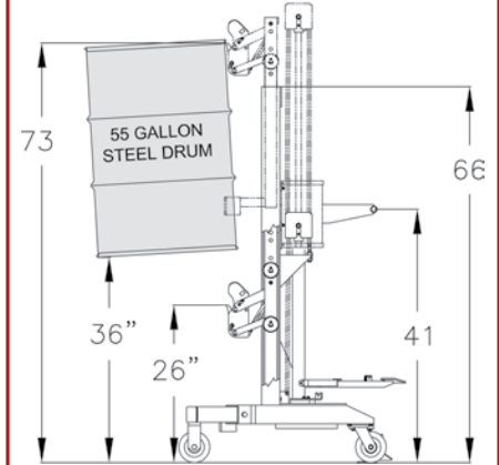
#240154 SCHEMATIC
