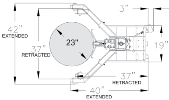
#240155 SCHEMATIC
