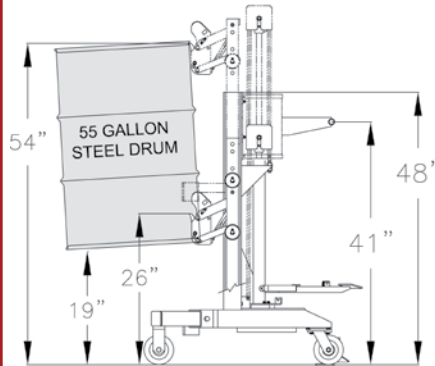
#240150 SCHEMATIC
