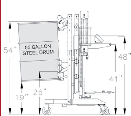
#240155 SCHEMATIC
