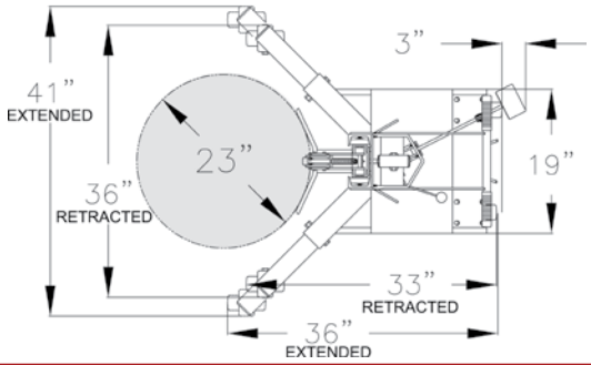
#240150 / #240154 SCHEMATIC
