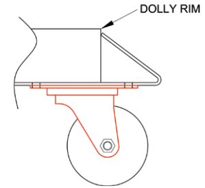
Drum Dolly Part #240197 / Model #SS5-PPSS All stainless rigs with 3" polypropylene wheels
