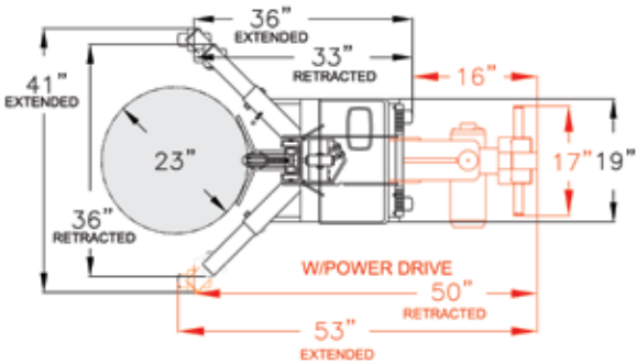
#240156 / #240157 SCHEMATIC
