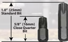
VHC77 Close Quarter Bits
