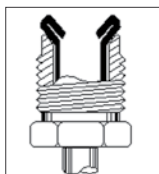
Flare tubing SAE (double) 7/16" – 24 thread
