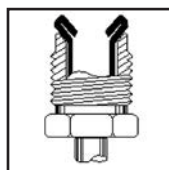
Flare tubing SAE (double) 7/16" - 24 thread
