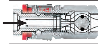
Unrestricted air flow - completely open
