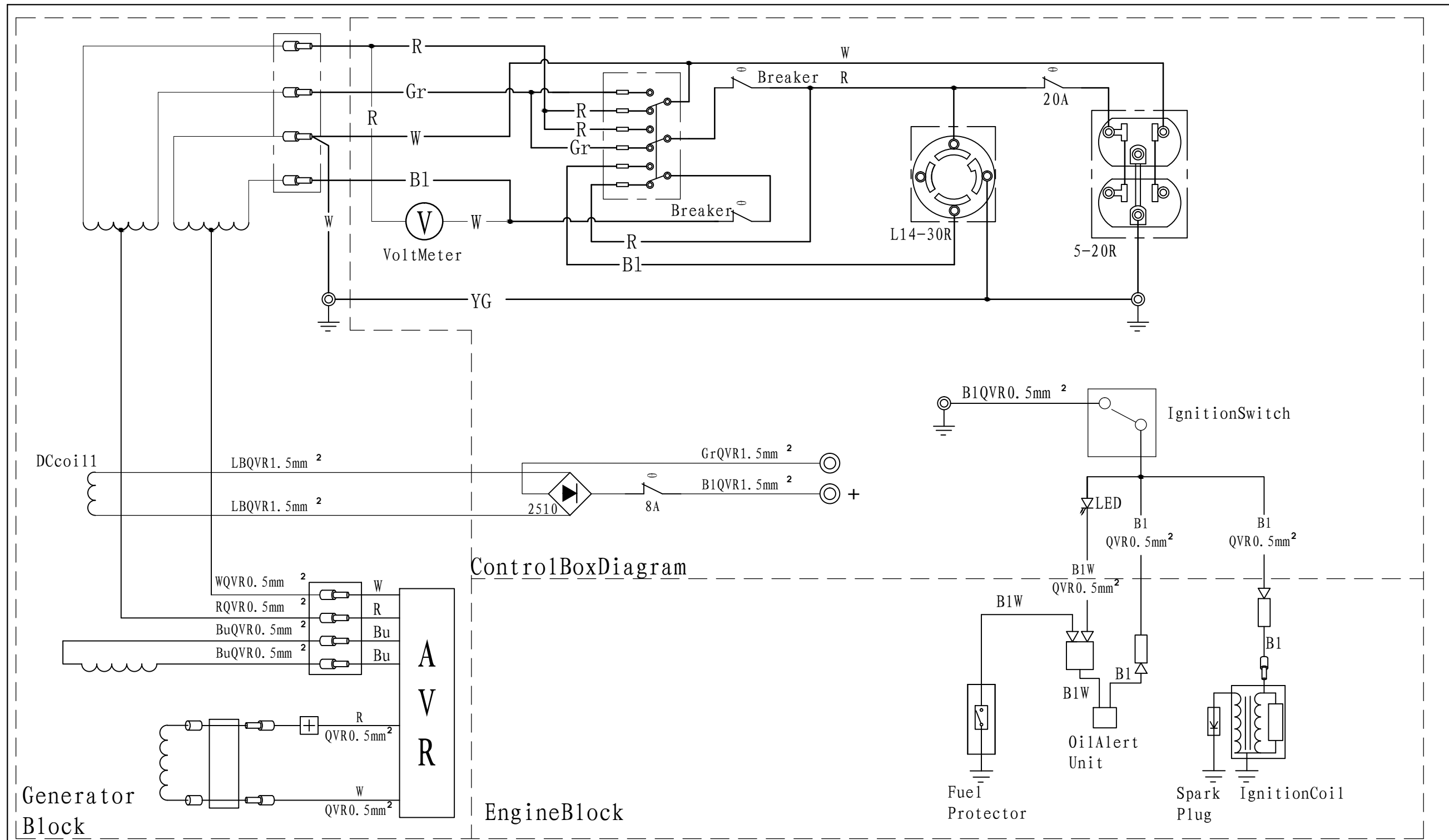
WIRING DIAGRAM OF 120V/240V GENERATOR SET PG3500
