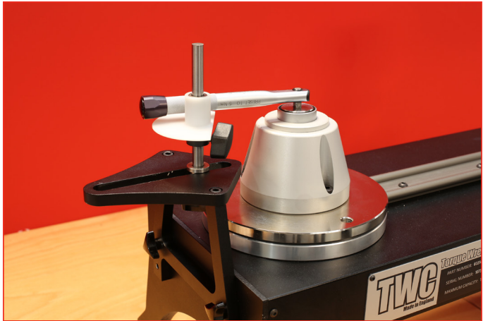
60318 Static Transducer Support Kit and 60319 Short Length Reaction Post
