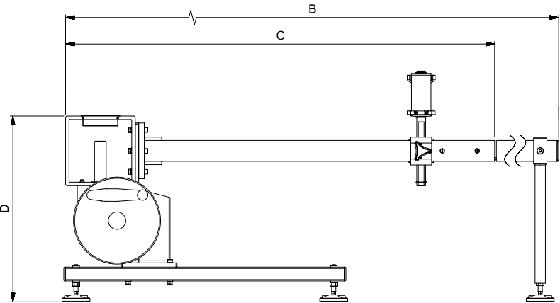
20506 ISO 3,000 N·m Motorised Loader
