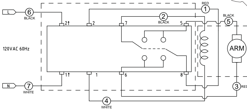
AC SWITCH 10A 125V AC with FWD/REV
