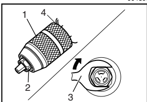
1. Sleeve 2. Hexagonal nut 3. Wrench 19 4. Retaining ring
