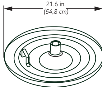
278965 follower 400 lb. (181 kg) drum Ultra high pressure PowerMaster
