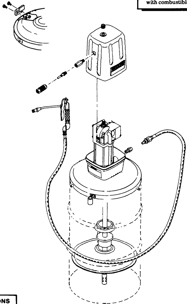
917-57 PORTABLE LUBRIGUN
