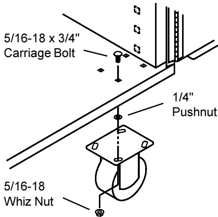
Figure 3. Caster Mounting
