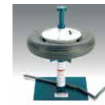
Threadscrew has been milled to fit MTD wheels.
