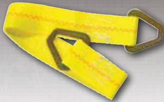
04223 24" x 2" Axle Strap w/D-Ring 1,666 lbs. WLL 5,000 lbs. Break Strength Package: Clamshell Ship Pack 4
