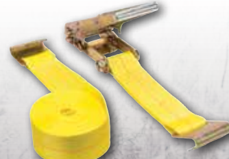
04637 27' x 3" Ratchet Tie-Down 5,000 lbs. WLL 15,000 lbs. Break Strength
