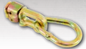
89304 O-Track Double Stud Fitting 2,000 lbs WLL 6,000 lbs. Break Strength Package: Bulk/Cut Case Ship Pack 12
