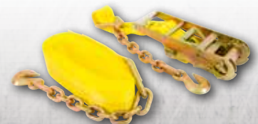
04655 30' x 3" Ratchet Tie-Down w/Chain Ends & Grab Hook 5,000 lbs. WLL 15,000 lbs. Break Strength
