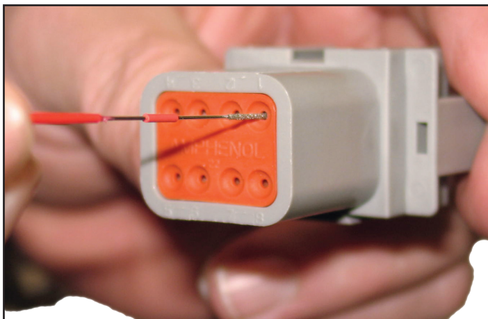
Smallest File (.030") Shown (Above) Cleaning a Connector
