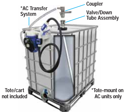
#DEFSSV Stainless Steel Tote Valve and Down Tube Kit
