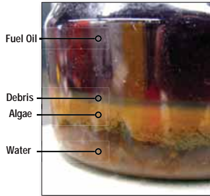
Sample Oil Removed from Tank
