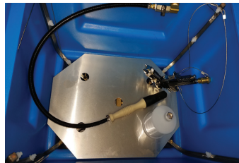
G202 tank with brush
