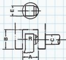
Ball Anvil
