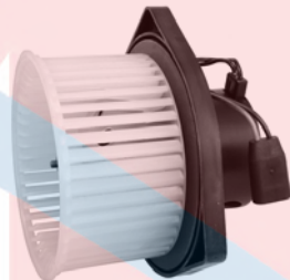
35085 CW 2 Lead Wires w/ connector Style: Flanged Voltage: 12 Buick (07-05); Chevy (09-01); Olds (04-01); Pontiac (09-01), (98-97); Saturn (07-05) General Motors Corp: 15249638
