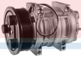
68619 New TM21HD 8 Groove 12 Volt Pulley Dia.: 5 Coil Clock: Wire Lead Seltec: 10367260, 43567260, 48867260 Western Star: 3006971
