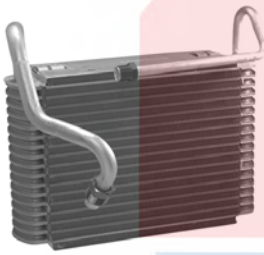
54401 Plate & Fin Evaporator Core O-Rings: (1) 24608 , (1) 24612 , (1) 38623 Chevy (84-80); GMC (84-80)
