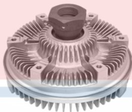
46035 STD Severe Duty GMC & CHEVY (02-01) General Motors Corp: 15030120, 15764819, 15768378
