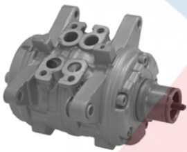
57360 Reman 10P13A May Require use of OE Manifold Mount: Ear Mount Chrysler (91); Mazda (92-88)
