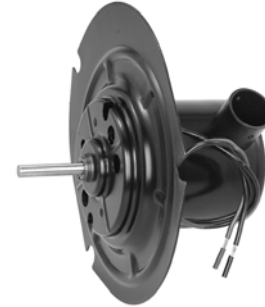
35650 CCW 2 Lead Wires Style: Flanged Voltage: 12 Dodge (78-72) Euclid: E803085
