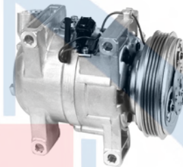
68442 New 67442 Reman DKV14C 4 Groove 12 Volt Switch: Heat Sensor Pulley Dia.: 4-3/4 Coil Clock: Wire Lead Nissan (99-98)
