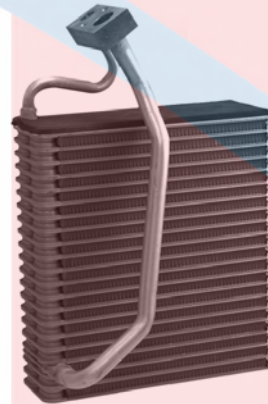
54710 Plate & Fin Evaporator Core Inlet: Block Fitting Outlet: Block Fitting O-Rings: (1) 24149 Chrysler (00-95); Dodge (00-95); Plymouth (00-96) Depth Height Width 3 13-5/8 5
