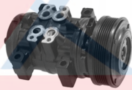
57365 Reman 10P15F May Require use of OE Manifold 6 Groove 12 Volt Mount: Tangent Mount Belt Width: 7/8 Pulley Dia.: 5 Coil Clock: Wire Lead New Clutch Assy: 47853 Reman Clutch Assy: 48853 Ford (95-89)
