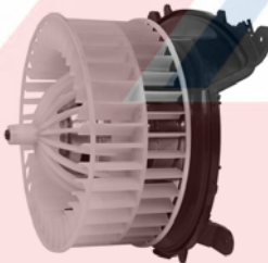
76972 CCW 2 Lead Wires w/ Connector Style: Flanged Voltage: 12 Mercedes (06-00) Mercedes Benz: 2208203142
