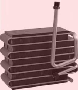
54185 Serpentine Evaporator Core O-Rings: (1) 24608 , (1) 24610 Mazda (98-94)
