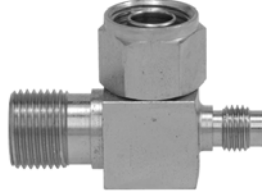
12194 Compressor Discharge (R12) 90° Connector A Size: 8 Connector B Size: 8 Bergstrom: 540223 Climatech: AB3300 Euclid: E80802310 Kysor: 1408047 NaviStar: 706024
