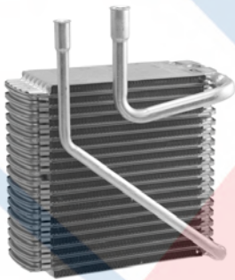
54548 Plate & Fin Evaporator Core O-Rings: (1) 24608 , (1) 24610 Ford (03-91); Mercury (99-91)
