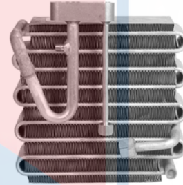
54691 Serpentine Evaporator Core Outlet: Block Fitting O-Rings: (1) 24604 , (1) 24604 , (1) 24608 , (1) 24610 Honda (93-92)
