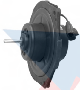
35252 CCW 2 Lead Wires Style: Flanged Voltage: 12 Chevy (02-98) General Motors Corp: 52486805
