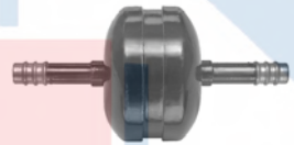
34248 Beadlock In-Line Filter w/ Desiccant for Liquid Line Outside Dia.: 2.500 Length: 3.000 Inlet Fitting Type: Barb Fitting Outlet Fitting Type: Barb Fitting Euclid: E8047088 Northern: 804312
