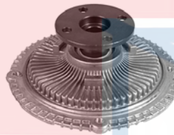
36984 STD Standard Duty Nissan (88-84) Nissan: 2108217C15, 2108217C16, 21082W4405
