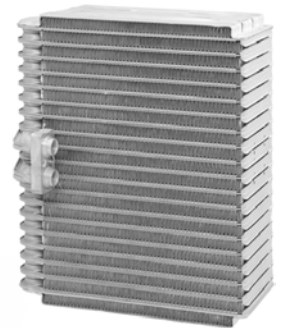
54730 Depth Height Width 3-9/16 10-1/2 5 Plate & Fin Evaporator Core Inlet: Block Fitting Outlet: Block Fitting O-Rings: (2) 24610 Toyota (04-95) Toyota: 8850104030
