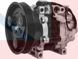
58487 New 57487 Reman N1301AE4 5 Groove 12 Volt Switch: Switch Mount: Tangent Mount Pulley Dia.: 5-1/4 Coil Clock: Wire Lead Ford (97-93); Mazda (97-93) Mazda: GA2A61450, GB6H61450D
