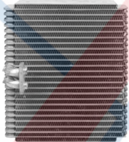
54721 Plate & Fin Evaporator Core Inlet: Block Fitting Outlet: Block Fitting O-Rings: (2) 24682 Acura (95-91) Acura: 80210SP0A01
