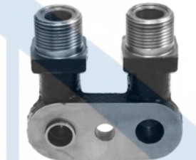
12201 Adapter Compressor Suction and Discharge Euclid: E808495 Red Dot: 75R8520
