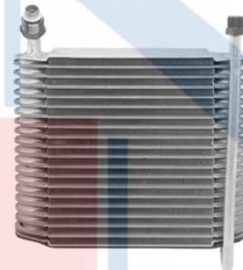
54598 Depth Height Width 2-7/8 12-7/8 3-3/8 Plate & Fin Evaporator Core O-Rings: (1) 24608 , (1) 24612 Cadillac (00-99); Chevy (02-94); GMC (02-94)
