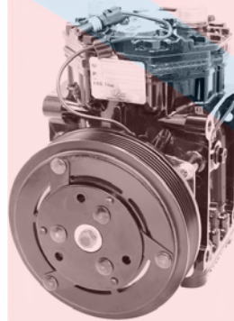
58025 New CCI 209/210 6 Groove 12 Volt Mount: Case Mount Pulley Dia.: 5-3/4 Coil Clock: Wire Lead Navistar: ET210L25078C
