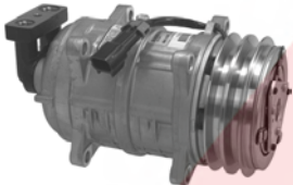
68173 New TM16 2 Groove 12 Volt Pulley Dia.: 4-3/4 Coil Clock: Wire Lead
