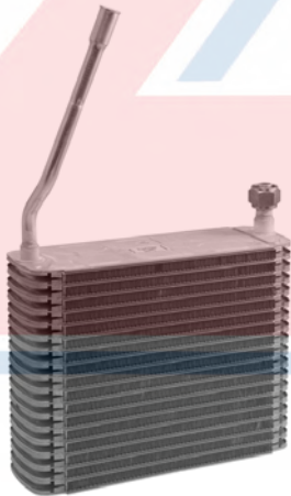
54549 Plate & Fin Evaporator Core O-Rings: (2) 24608 , (1) 24610 , (1) 38621 Ford (97-92); Lincoln (97-91); Mercury (97-92)
