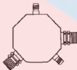
33152 Accumulator Outside Dia.: 3.500 Length: 9.000 Inlet Fitting Type: Dual O-Ring Inlet Fitting: 3/4" Outlet Fitting Type: Dual O-Ring Outlet Fitting: 3/4" O-Rings: (1) 24222 , (3) 24672 , (2) 24650 General Motors Corp: 2724875
