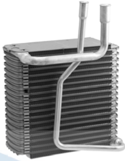
54546 Plate & Fin Evaporator Core O-Rings: (1) 24608 , (1) 24610 Ford (92-89)
