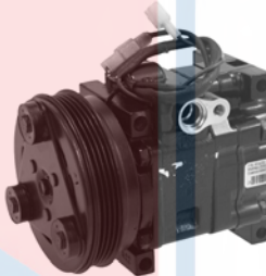
67470 Reman NL1300AE4 4 Groove 12 Volt Mount: Tangent Mount Pulley Dia.: 4-3/4 Coil Clock: Wire Lead Ford (97-94); Mazda (95)
