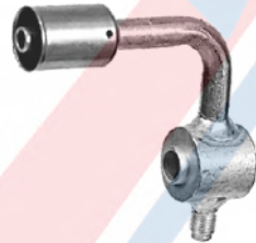
12055 Compressor Discharge (R12) Connector A Size: 8 Dallas Truck AC: 0956251BL Red Dot: 75R5838
