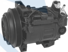
67665 Reman DCS17E 4 Groove 12 Volt Switch: Control Valve Pulley Dia.: 5-1/4 Coil Clock: Wire Lead Infiniti (08-06) Infiniti: 92600EG00C
