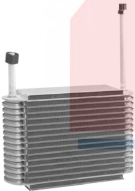
54535 Depth Height Width 4 15-7/16 4 Plate & Fin Evaporator Core O-Rings: (1) 24608 , (1) 24610 , (1) 38623 Ford (94-83); Mazda (94-91)
