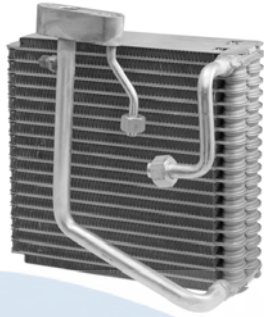
54296 Plate & Fin Evaporator Core Inlet: Block Fitting Outlet: Block Fitting O-Rings: (1) 24604 , (1) 24629 Acura (01-98); Honda (06-97) Honda: 80215ST3G01, 80215ST3G11
