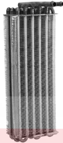
54135 Tube & Fin Evaporator Core Inlet: Block Fitting O-Rings: (1) 24608 , (1) 24610 Mercedes (93-84) Mercedes Benz: 0008305158
