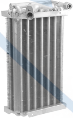
54664 Depth Height Width 2-1/2 13-7/8 7-1/2 Tube & Fin Evaporator Core Outlet: Block Fitting O-Rings: (1) 24608 , (1) 24610 Porsche (95-85)
