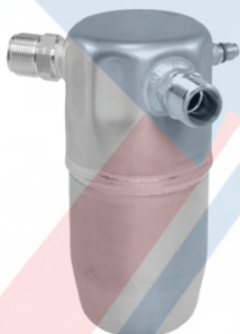
33130 Accumulator Outlet Fitting: 3/4" Buick (91); Olds (91); Pontiac (93-92)
