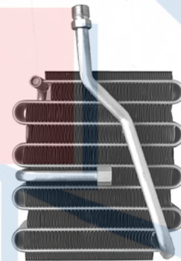
54151 Depth Height Width 3-15/16 4 Serpentine Evaporator Core O-Rings: (1) 24608 , (1) 24610 Toyota (85-81) Toyota: 8850114090, 8850114192
