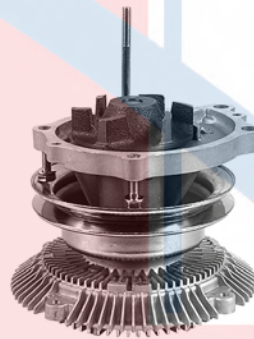
36983 STD Standard Duty Nissan (89-74) Nissan: 21010G3928, 21010N5885, BA01080W89
