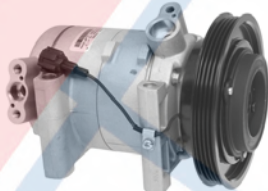
68428 New 67428 Reman 67429 Reman DKV14C 4 Groove 12 Volt Switch: Heat Sensor Pulley Dia.: 5-5/8 Coil Clock: Wire Lead Nissan (04-99) Nissan: 926007B410
