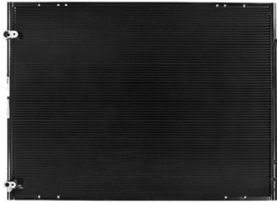
40243 Parallel Flow Lexus (09-07) Lexus: 884600E020
