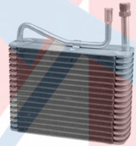
54551 Depth Height Width 3-9/16 11-5/8 3-9/16 Plate & Fin Evaporator Core O-Rings: (1) 24610 , (2) 24608 Lincoln (92-88); Mercury (88-87)
