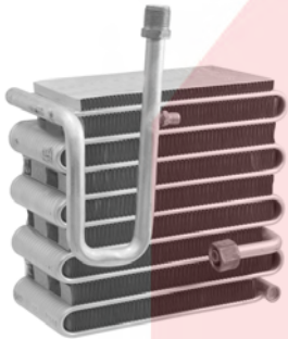
54702 Serpentine Evaporator Core O-Rings: (1) 24608 , (1) 24610 Mazda (89-86) Depth Height Width 3-7/8 11-7/16 6-1/4
