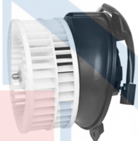
75741 CCW 2 Lead Wires w/ connector Style: Flanged Voltage: 12 Chrysler (04-99); Dodge (04-99) Chrysler: 4596217, 4885148AC
