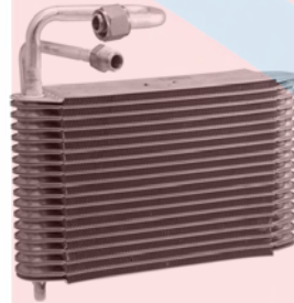
54411 Plate & Fin Evaporator Core O-Rings: (1) 24682 , (1) 23680 Buick (91-89); Cadillac (91); Olds (91-89); Pontiac (91-89) General Motors Corp: 52450552
