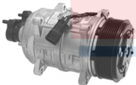
68175 New TM16 8 Groove 12 Volt Pulley Dia.: 4-11/16 Coil Clock: Wire Lead
