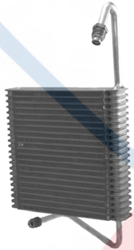
54588 Depth Height Width 2-7/8 19-3/4 5-3/8 Plate & Fin Evaporator Core O-Rings: (1) 24608 , (2) 24612 , (1) 38623 Chevy (98-96); GMC (98-96)
