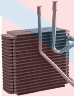
54792 Plate & Fin Evaporator Core O-Rings: (3) 24668 , (3) 24670 Ford (03-95) Ford: F58Z19850BA
