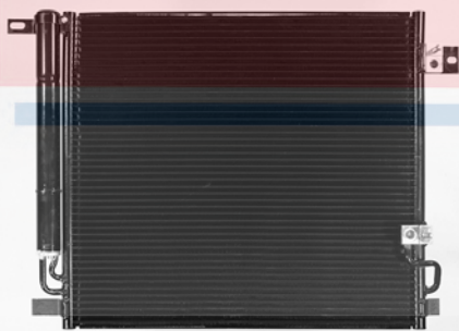
40202 Parallel Flow Chevy (12-09); GMC (12-09) General Motors Corp: 25964057
