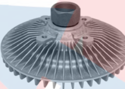
36974 REV Standard Duty Ford (96-87) Ford: F3TZ8A616C
