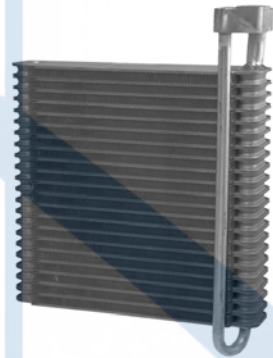
54573 Depth Height Width 2-7/8 14-1/4 3-5/8 Plate & Fin Evaporator Core Inlet: Block Fitting Outlet: Block Fitting O-Rings: (1) 24402 , (1) 24404 Chevy (02-99); GMC (02-99)
