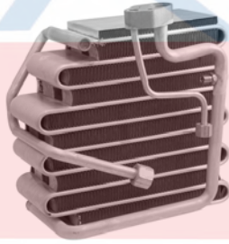
54670 Serpentine Evaporator Core Outlet: Block Fitting O-Rings: (1) 24608 , (1) 24612 , (1) 24616 Mitsubishi (93-92)
