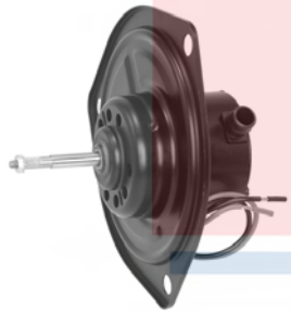
35631 CW/CCW 2 Lead Wires w/ Connector Style: Flanged Voltage: 12 Dodge (86-85); Plymouth (86-85); Toyota (86-79) Toyota: 8710414090, 8710422110, 8710432020
