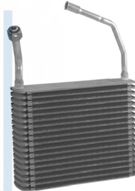
54795 Plate & Fin Evaporator Core O-Rings: (1) 24610 , (2) 24668 , (1) 38635 Ford (09-01); Mazda (09-02) Ford: 1L5Z19850FC Mazda: 1F2161J41B
