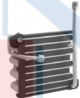
54719 Serpentine Evaporator Core O-Rings: (1) 24604 , (1) 24608 , (1) 24610 Mitsubishi (96-94)
