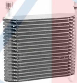
54431 Depth Height Width 2-7/8 13-1/8 3-1/4 Plate & Fin Evaporator Core O-Rings: (1) 24608 , (1) 24612 , (1) 38623 Chevy (90-88); GMC (90-88)
