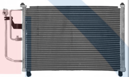
40034 Parallel Flow Daewoo (02-99) Daewoo: 96274635
