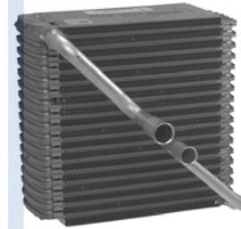
54717 Plate & Fin Evaporator Core O-Rings: (3) 24668 , (3) 24670 Hyundai (93-89)
