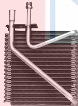
54555 Plate & Fin Evaporator Core O-Rings: (1) 24608 , (1) 24670 Ford (97-93)
