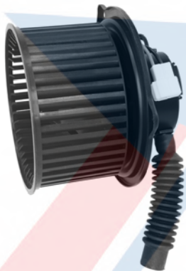
35079 CCW 2 Lead Wires w/ connector Style: Flanged Voltage: 12 Hyundai (06-01); Kia (06-01) Hyundai: 971132D010 Kia: 971123F000
