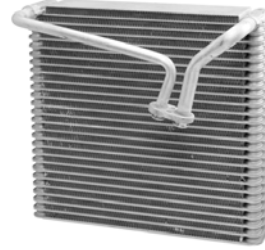
54690 Serpentine Evaporator Core Inlet: Block Fitting O-Rings: (1) 24661 , (1) 24681 Acura (06-01); Honda (08-99)
