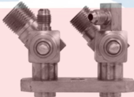
12185 Adapter Compressor Suction and Discharge Connector A Size: 10 Connector B Size: 8
