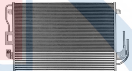
40286 Parallel Flow Ford (12-08); Mazda (11-08); Mercury (11-08) Ford: 8L8Z19712G
