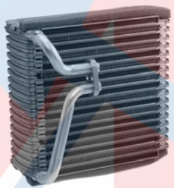
54723 Plate & Fin Evaporator Core Inlet: Block Fitting O-Rings: (2) 24608 Hyundai (99-98) Hyundai: 9760922001
