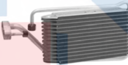
54417 Depth Height Width 2-7/8 8-3/4 4 Plate & Fin Evaporator Core Outlet: Block Fitting O-Rings: (2) 24606 , (1) 24403 , (1) 24404 Chevy (05-95); GMC (05-95)
