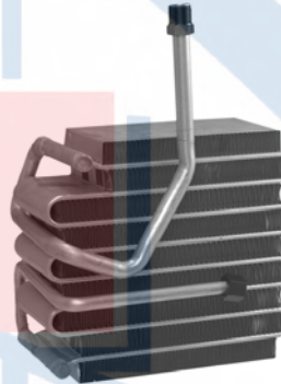
54682 Depth Height Width 4 13-1/4 6-5/8 Serpentine Evaporator Core O-Rings: (1) 24608 , (1) 24610 Toyota (88-84)
