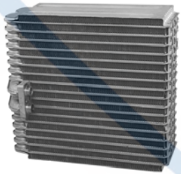
54299 Plate & Fin Evaporator Core Inlet: Block Fitting Outlet: Block Fitting O-Rings: (2) 24682 Toyota (02-94) Toyota: 8850102021
