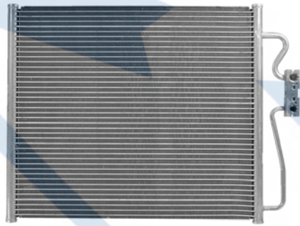
40551 Parallel Flow BMW (97-95) BMW: 64538373924
