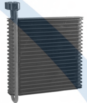
54467 Depth Height Width 2-7/8 13-3/4 3-3/4 Plate & Fin Evaporator Core Inlet: Block Fitting Outlet: Block Fitting O-Rings: (1) 24659 , (1) 24682 Buick (96-91); Cadillac (96-93); Chevy (96-91); Olds (92-85)
