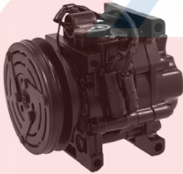
57496 Reman N1300AC4 1 Groove 12 Volt Mount: Ear Mount Belt Width: 7/16 Pulley Dia.: 5 Coil Clock: Wire Lead Subaru (89-88) Subaru: SOA438A265
