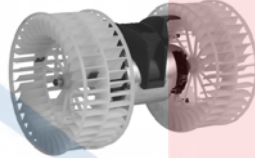
76975 CCWLE 2 Spade Terminals Style: Double Shaft Voltage: 12 Mercedes (95-86) Mercedes Benz: 0008308208
