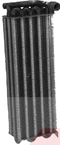
54430 Depth Height Width 3 15-7/8 6-1/2 Tube & Fin Evaporator Core O-Rings: (1) 24606 , (2) 24610 Chevy (91-88), (80-72); GMC (91-88), (84-72)
