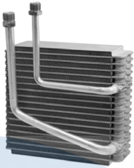
54784 Depth 3 Height 3-1/8 Width Plate & Fin Evaporator Core O-Rings: (1) 24608 , (1) 24610 Mazda (02-98) Mazda: GD7A61J10A
