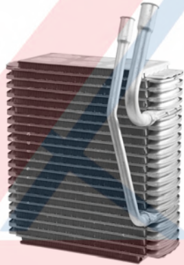
54569 Depth Height Width 3-9/16 13-1/8 6-1/4 Plate & Fin Evaporator Core O-Rings: (3) 24668 , (3) 24670 Dodge (94); Jeep (94-93)
