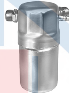
33156 Accumulator Outside Dia.: 3.500 Length: 8.000 Inlet Fitting Type: Dual O-Ring Outlet Fitting Type: Dual O-Ring O-Rings: (4) 24082 Cadillac (02-93) General Motors Corp: 2724914
