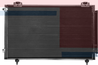
40067 Parallel Flow Toyota (04-03) Toyota: 8845002170, 8845012231
