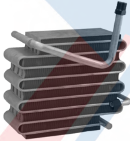
54669 Serpentine Evaporator Core O-Rings: (1) 24608 , (1) 24610 Dodge (89-87); Mitsubishi (91-83)
