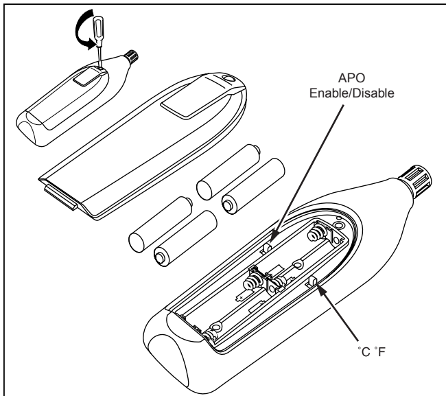
Figure 1. Battery Compartment
