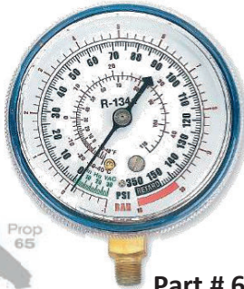
Part # 6133 R-134a Low Side Gauge
