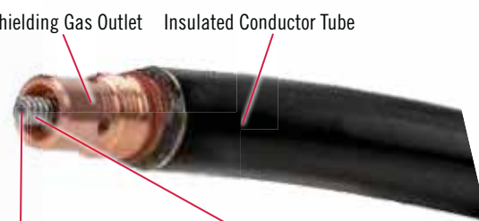
Perfectly Centered Liner
