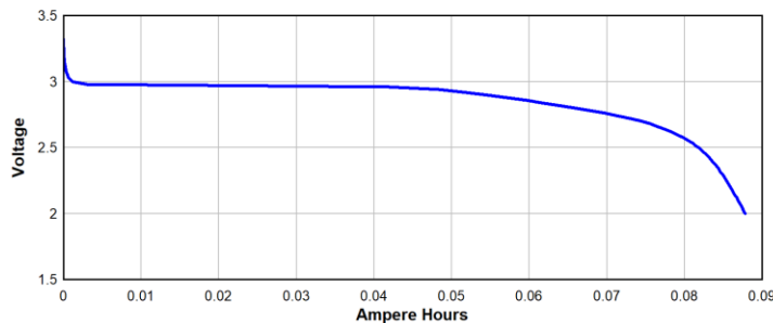
IEC Rated Capacity 47k Ohm Continuous to 2.0V
