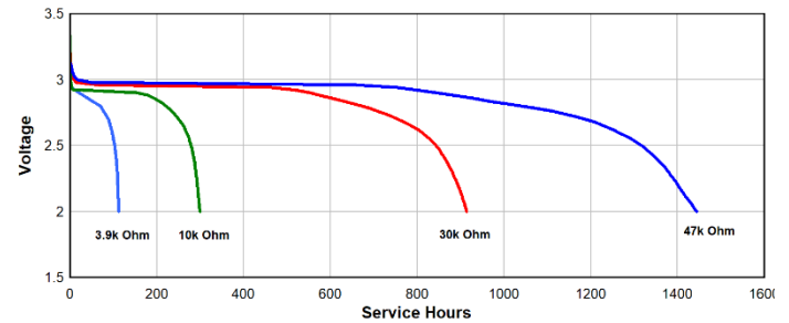
Continuous Discharge Multiple Loads to 2V
