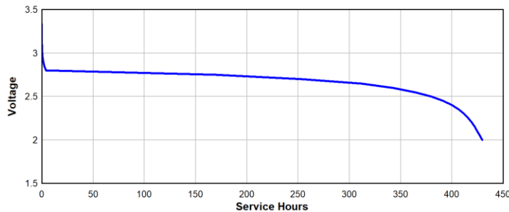
Cold Temperature Discharge 15k Ohm Continuous to 2V @ -10C
