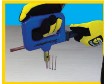
Pin Welding
