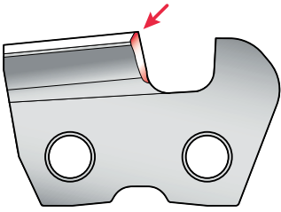
Too little top plate cutting angle
