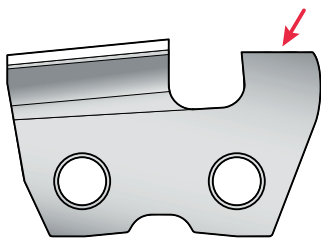
Square or blunt depth gauges
