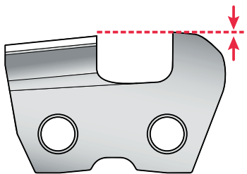
High depth gauges
