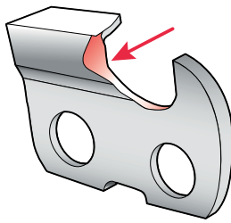
Severe abrasive damage on side plates
