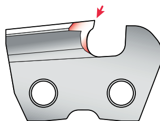
Too much hook in side plate
