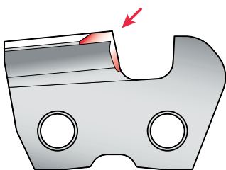
Too much top plate cutting angle
