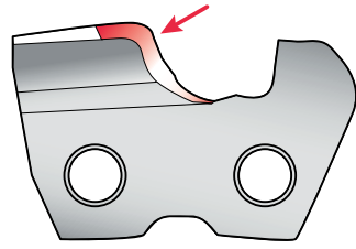
Backslope on side plate
