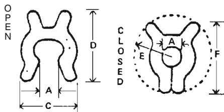
Commercial Tolerances All X-Washers
