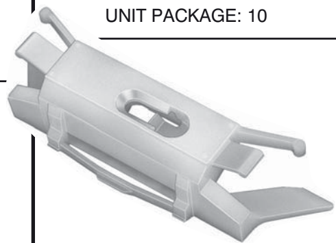
21094 (91572-SDA-A01) White Nylon Windshield Moulding Clip Width: 14mm Length: 62mm Accord 2003 - On Civic 2006 - On UNIT PACKAGE: 10
