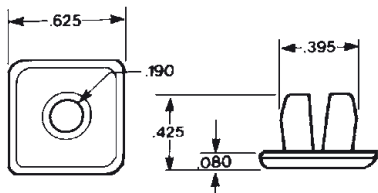
8435 (4755299) Nylon
