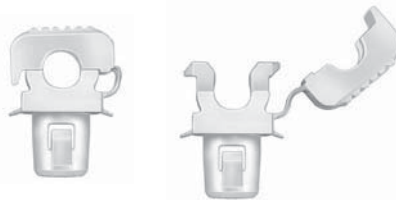
21336 (69293-30030) Natural Nylon
