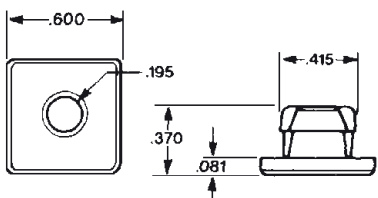
11719 (3907444) Nylon
