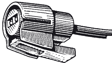
16514 (12085503) Replacement harness connector used on GM V-5 Air Conditioning Compressor Pressure Cut-off Switches. Fits GM low Pressure Switch 6551946 and others Index slot is at three o'clock position Features two 9" long 18 gauge wire leads UNIT PACKAGE: 1
