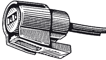
16513 (GM: 12085521) Replacement harness connector used on GM V-5 Air Conditioning Switches. Fits GM High Pressure Switch 6551917 and others. Index slot is at the one o'clock position. Features two 9" long 18 gauge wire leads. UNIT PACKAGE: 1
