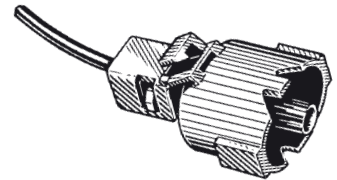
14580 (12102621) Radiator Fan Sensor Switch Harness Connector Fits electric cooling fan switches 3040674, 14043275 and 14043276. GM 1980-On UNIT PACKAGE: 1
