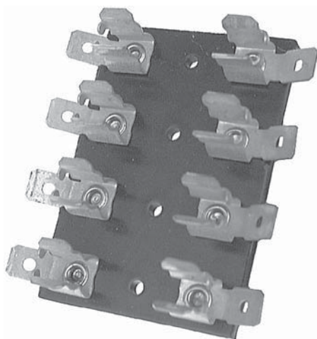
13445 Four Gang Fuse Block Size: 2-7/16" x 2-15/16" x 3/4" UNIT PACKAGE: 1
