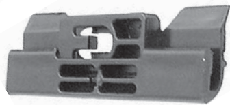
20387 (91519-S5A-003) Black Nylon Windshield Moulding Clip 17mm Wide, 50mm Long Upper Area Of Windshield Civic Coupe 2001 - On UNIT PACKAGE: 10
