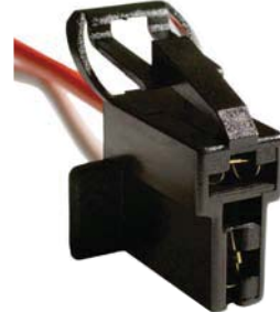
20838 (Not Supplied by O.E.M.) Alternator Harness Connector Two 16 Gauge Wire Leads 100 Amp Alternator Ford 1990 - 75 UNIT PACKAGE: 10
