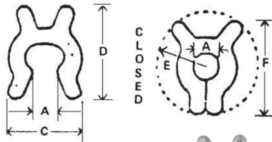
X-Washers Zinc
