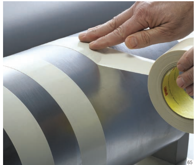
3M™ Traction Tape 5401 enhances friction on web rollers to help maintain constant traction and tension for the web material from start-up through wind-up.
